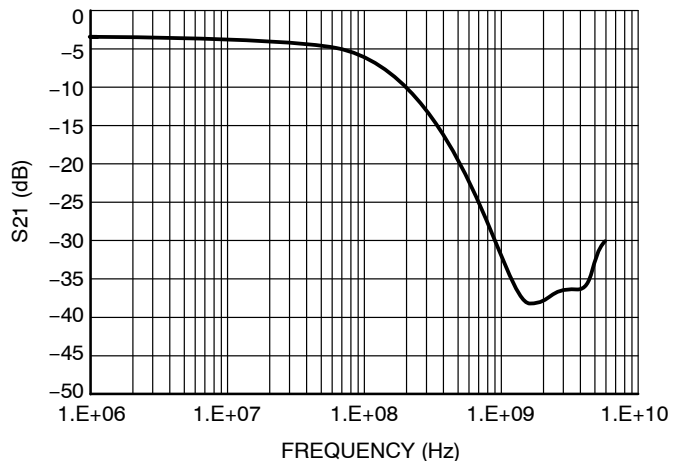
Figure 2. Insertion Loss Characteristic (S21 Measurement)
