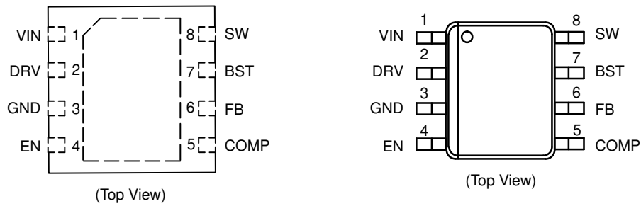
Figure 3. Pin Connections
