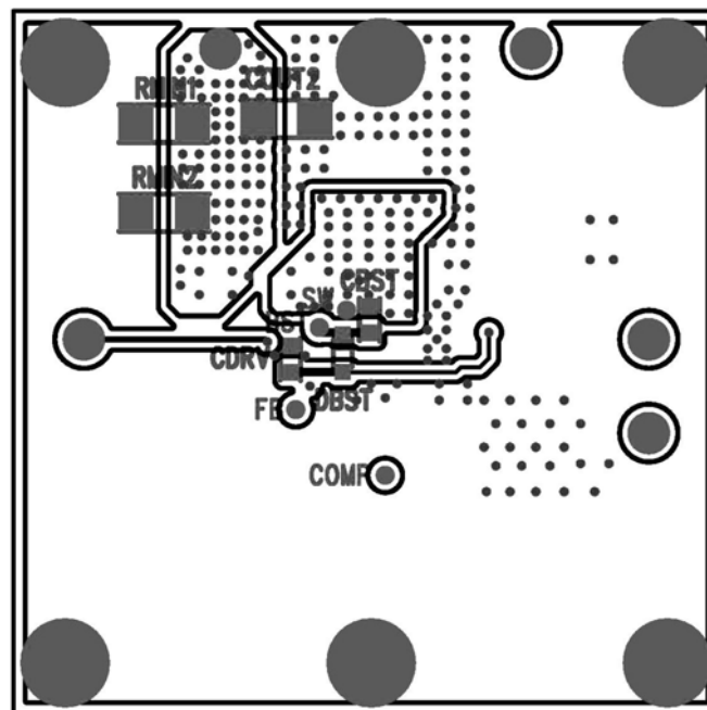
Figure 13. Bottom View
