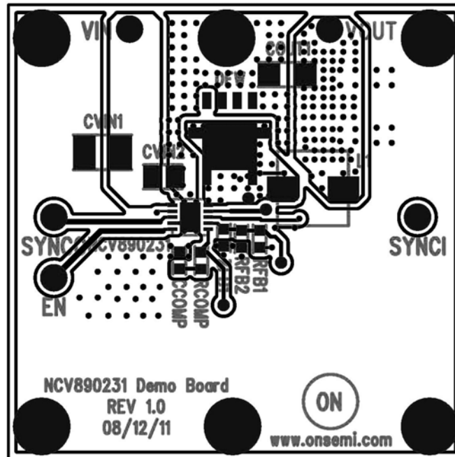
Figure 12. Top View
