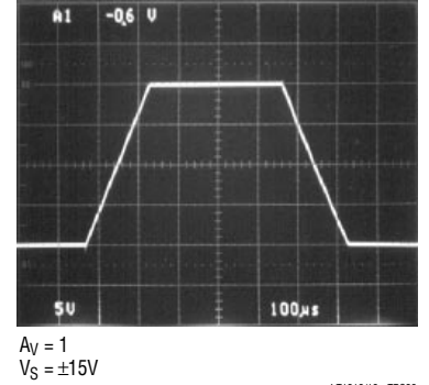
Large-Signal Response V_S = \pm 15\text{V}
