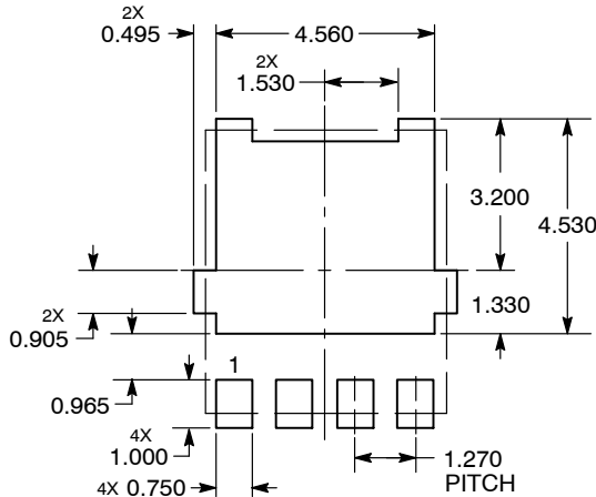
DIMENSIONS: MILLIMETERS
