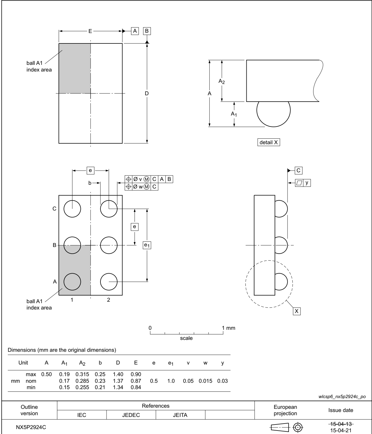
Fig 23. Package outline NX5P2924C
