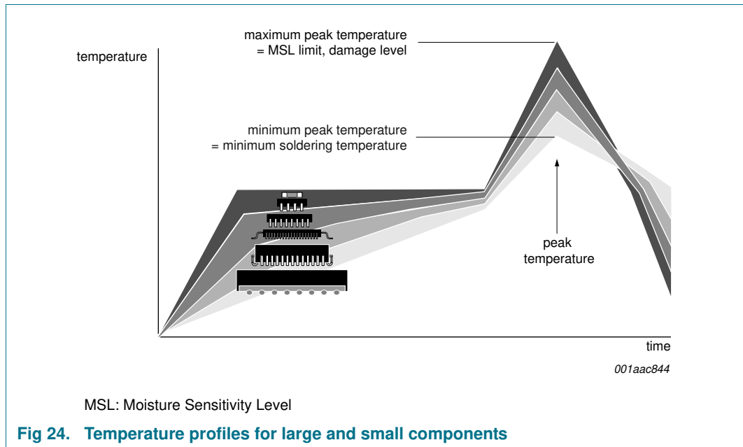
Fig 24. Temperature profiles for large and small components For further information on temperature profiles, refer to application note AN10365 “Surface mount reflow soldering description”.
