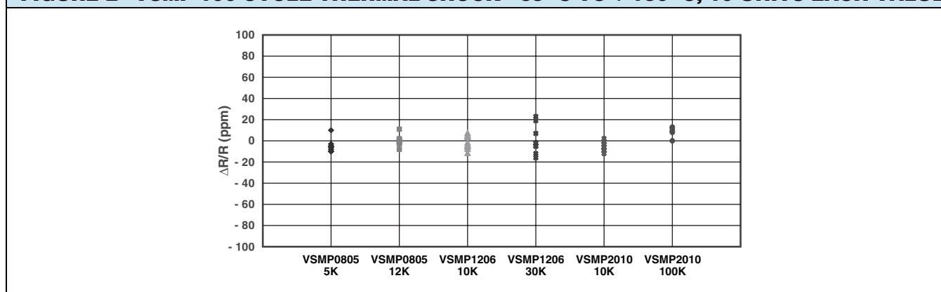
FIGURE 2 - VSMP 100 CYCLE THERMAL SHOCK - 65 °C TO + 150 °C, 10 UNITS EACH VALUE
