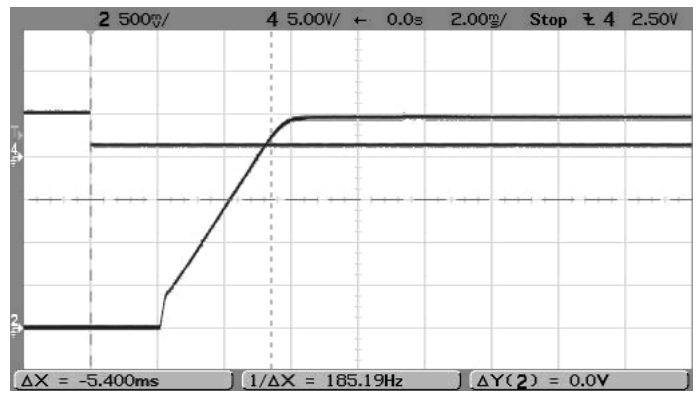
On/Off Enable Startup (V in =5V, V out =2.5V, I out =6A, Cload=0) Trace 4=Enable, Trace 2=Vout
