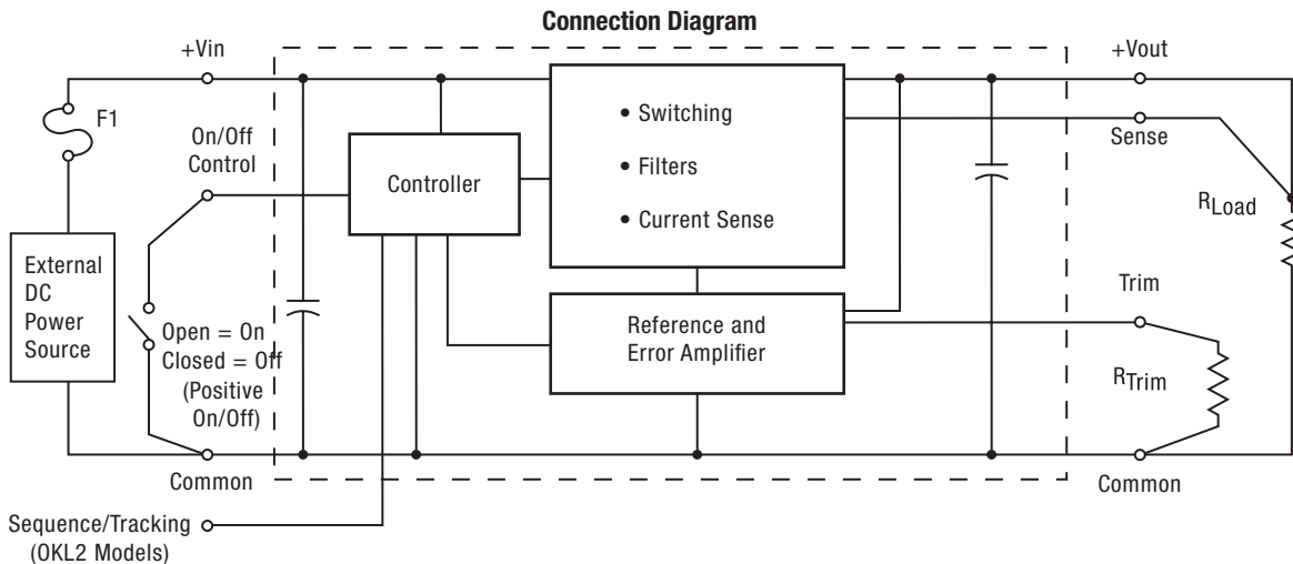
Figure 1. OKL-T/6-W5
