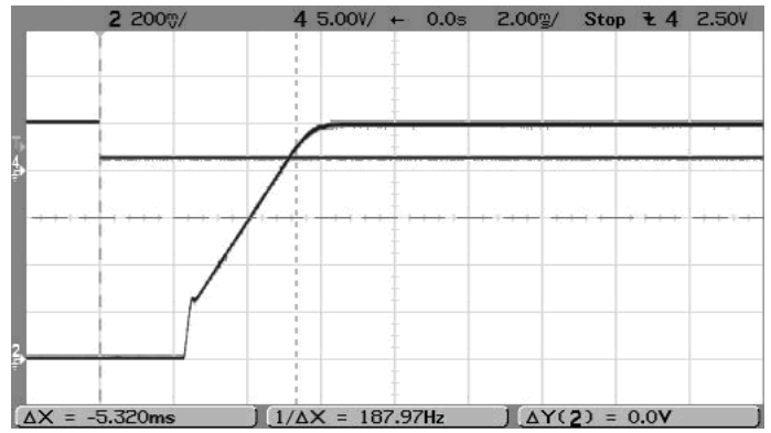
On/Off Enable Startup (V in =5V, V out =1.0V, I out =6A, Cload=0) Trace 4=Enable, Trace 2=Vout
