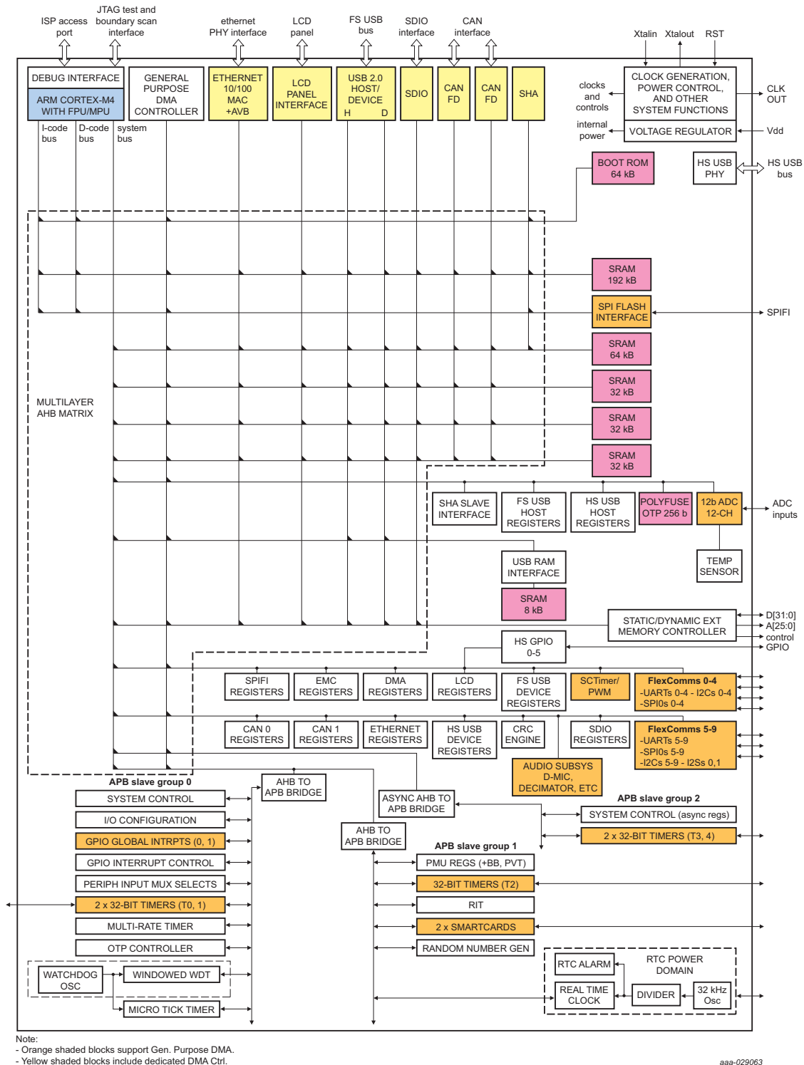
Fig 4. LPC540xx Block diagram
