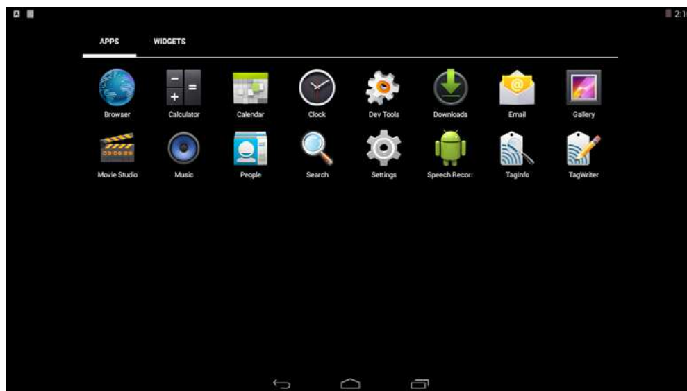
Fig 14. Android applications
