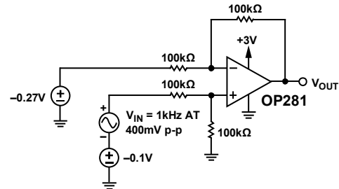
Figure 37. Single OPx81 Channel Configured as a Difference Amplifier Operating at V_{CM} < 0\text{V}
