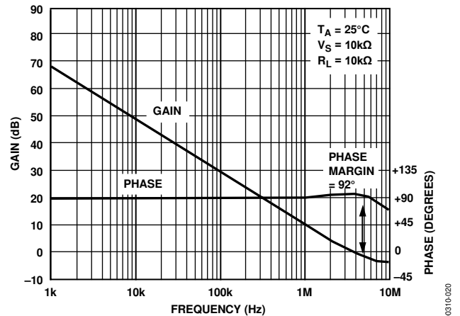
Figure 20. OP292/OP492 Open-Loop Gain and Phase vs. Frequency @ ±15 V
