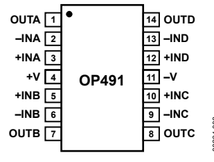
Figure 3. 14-Lead Narrow-Body SOIC
