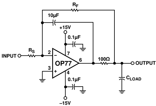
Figure 28. Isolating Large Capacitive Loads
