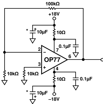
Figure 24. Burn-In Circuit
