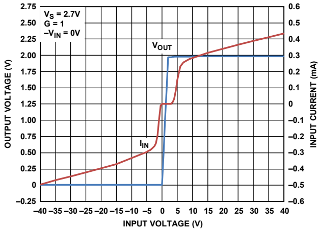
Figure 16. Input Overvoltage Performance, Single Supply, V_S = 2.7\text{ V} , G = 1
