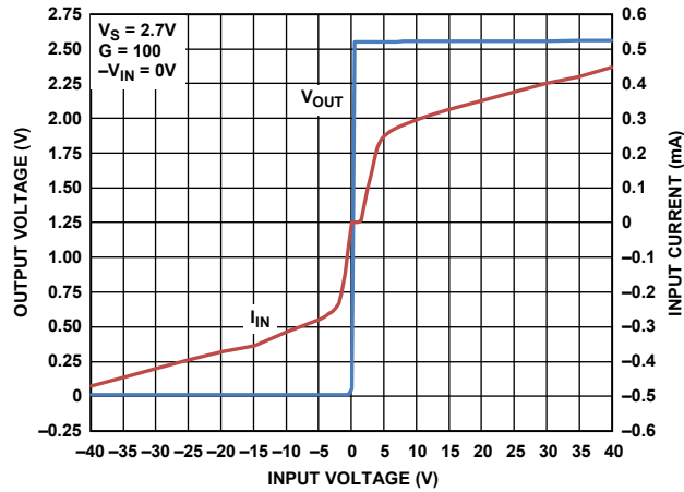
Figure 19. Input Overvoltage Performance, Single Supply, V_S = 2.7\text{ V} , G = 100
