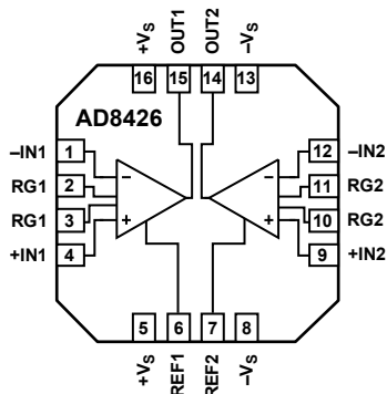
Figure 63. Pinout Diagram
