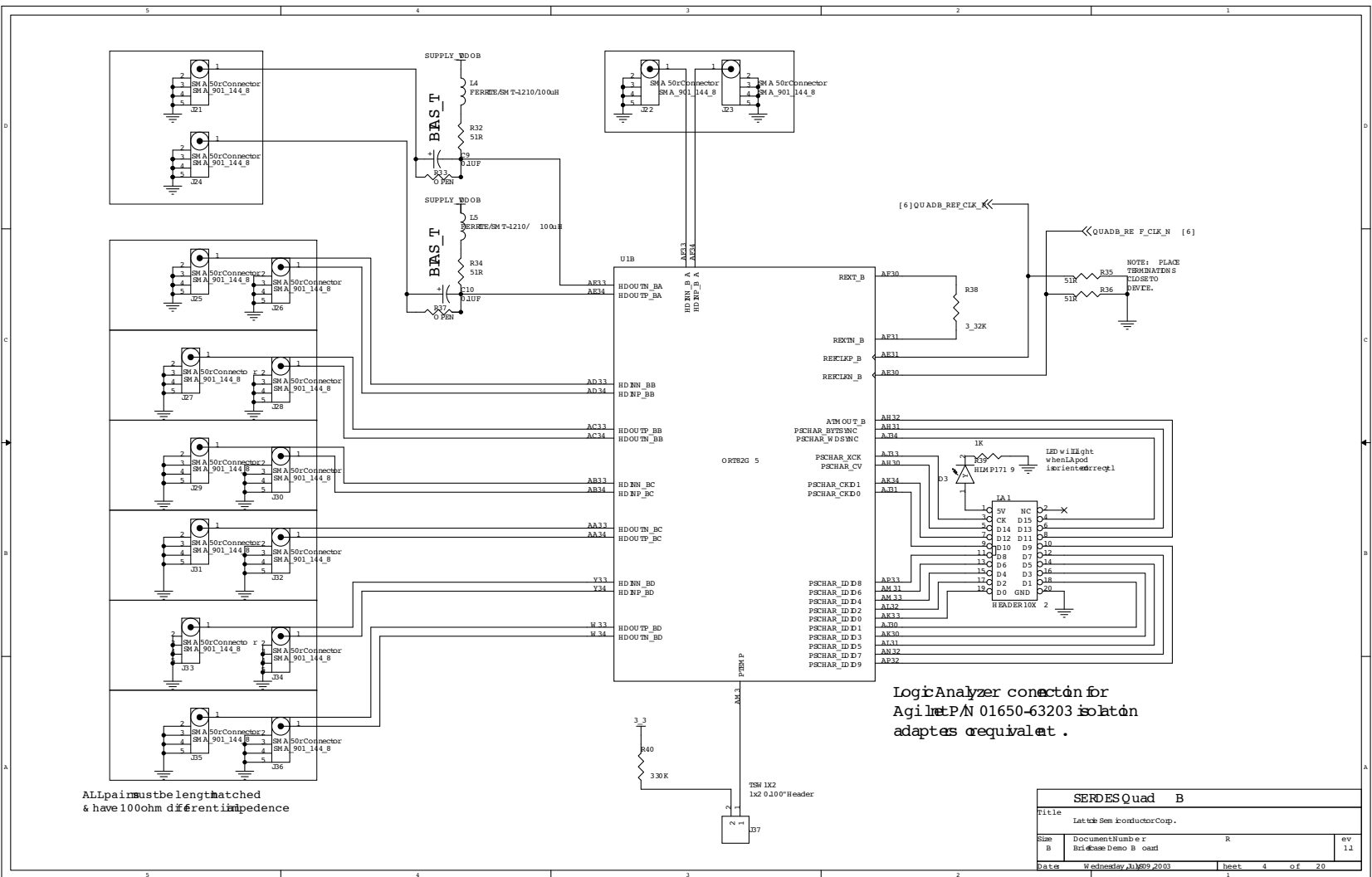
Figure 8. Lattice High-Speed SERDES Briefcase Board Schematic
