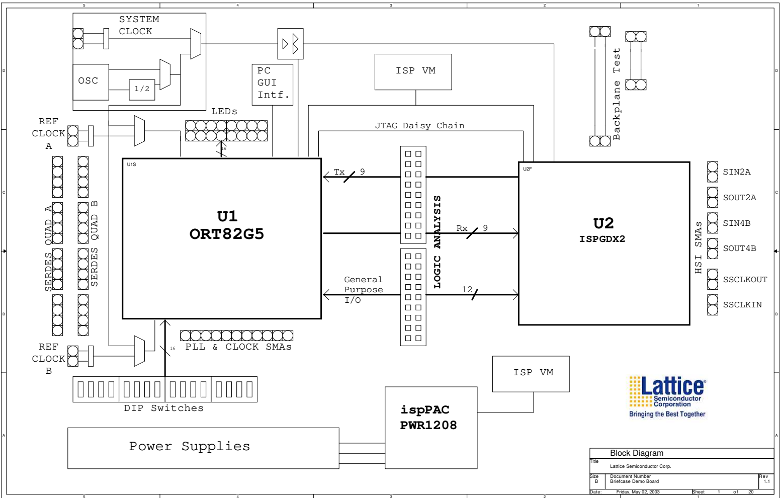
Figure 5. Lattice High-Speed SERDES Briefcase Board Schematic
