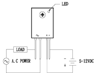
Fig.8 WIRING DIAGRAM
