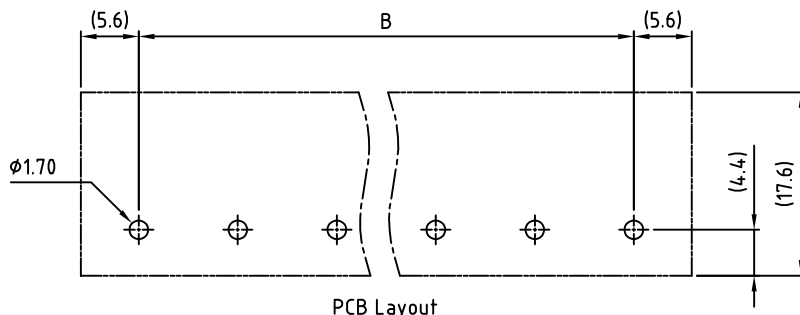
PCB Layout
