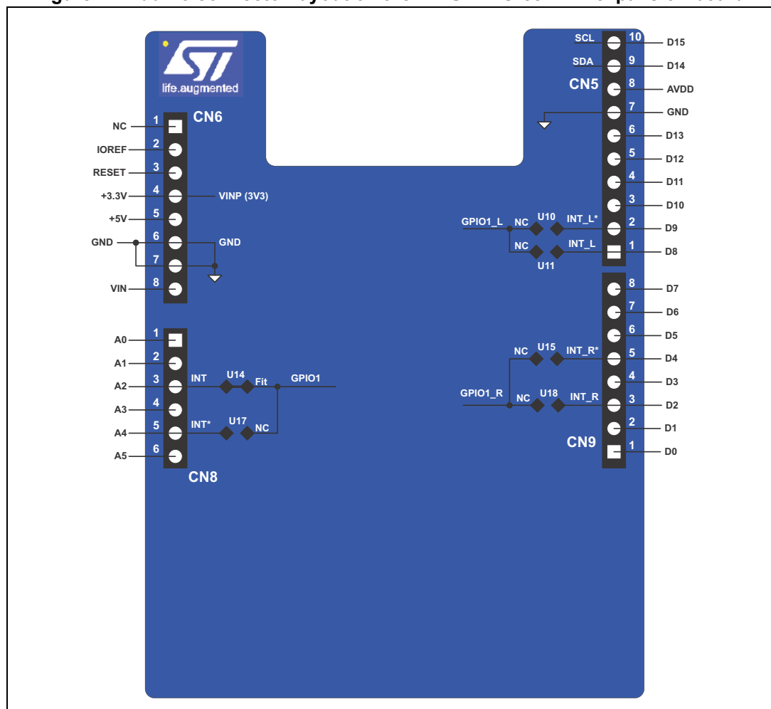
Figure 1. Arduino connector layout on the X-NUCLEO-53L1A1 expansion board
