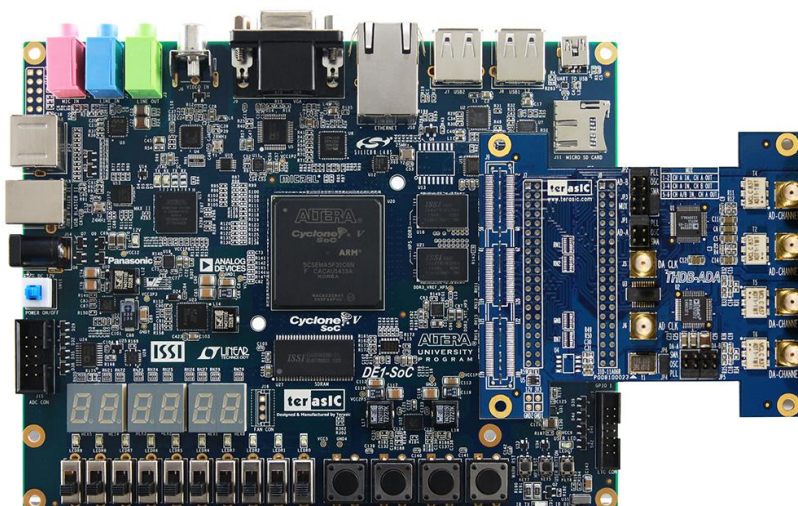
Figure 1-11 Connect ADA-GPIO with DE1-SoC
