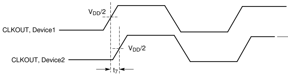
Figure 8. Device-Device Skew
