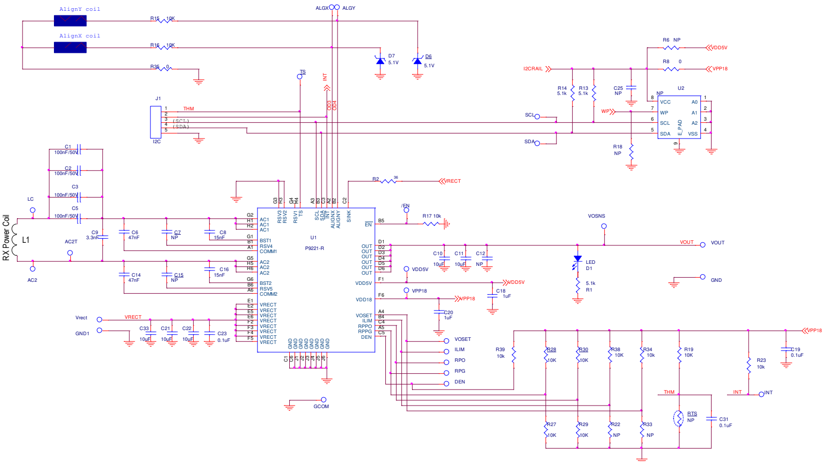
P9221-R MM EV Board V2.1
