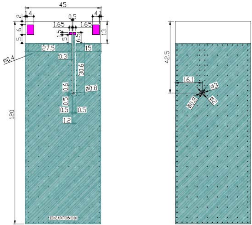
Figure 16. EVB Dimensions of the PA700J.
