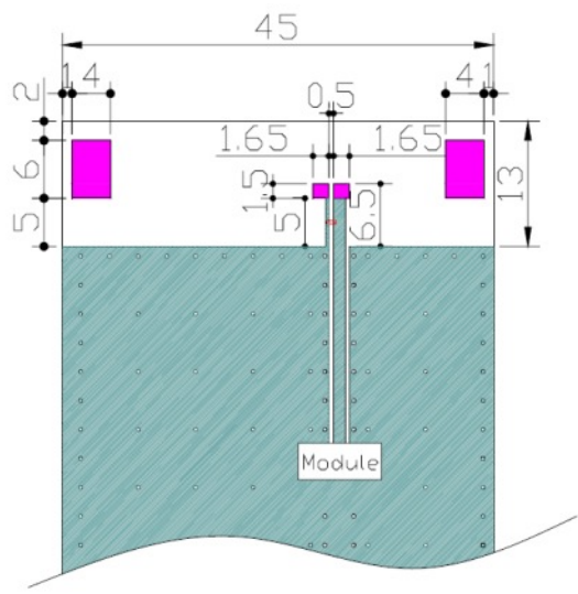
Figure 15. Layout dimensions of the PA700J Antenna.
