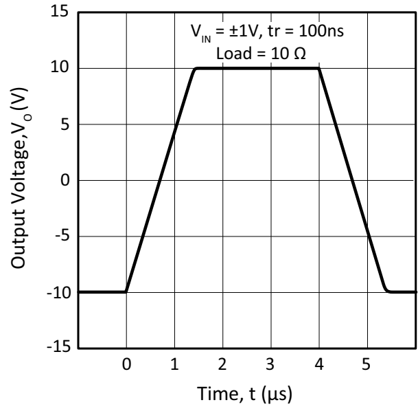
Figure 18: Loading Effects
