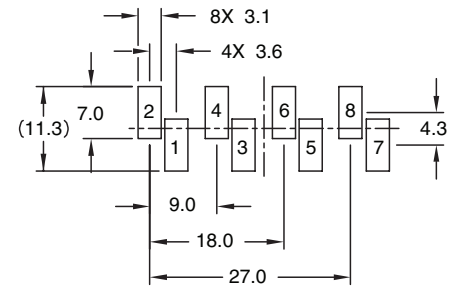
SUGGESTED LAND PATTERN TOLERANCE ON PADS = ± 0.05
