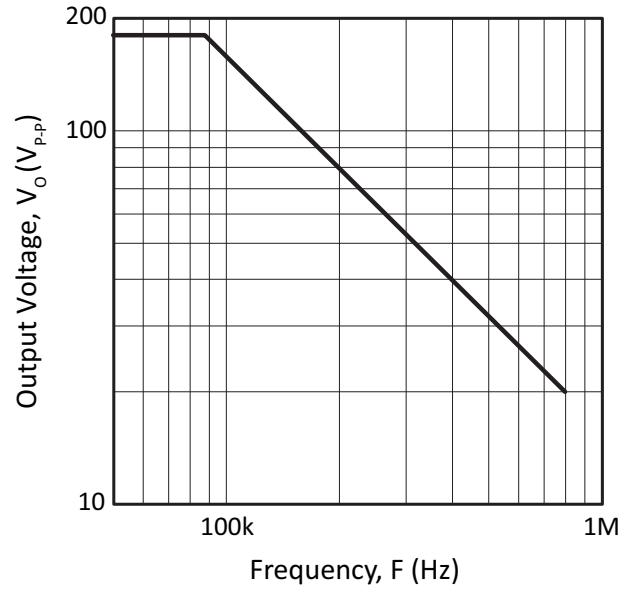
Figure 9: Power Response
