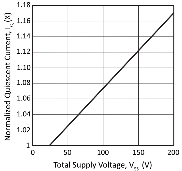
Figure 11: Quiescent Current
