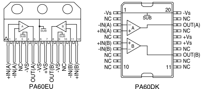
FIGURE 3. External connections
