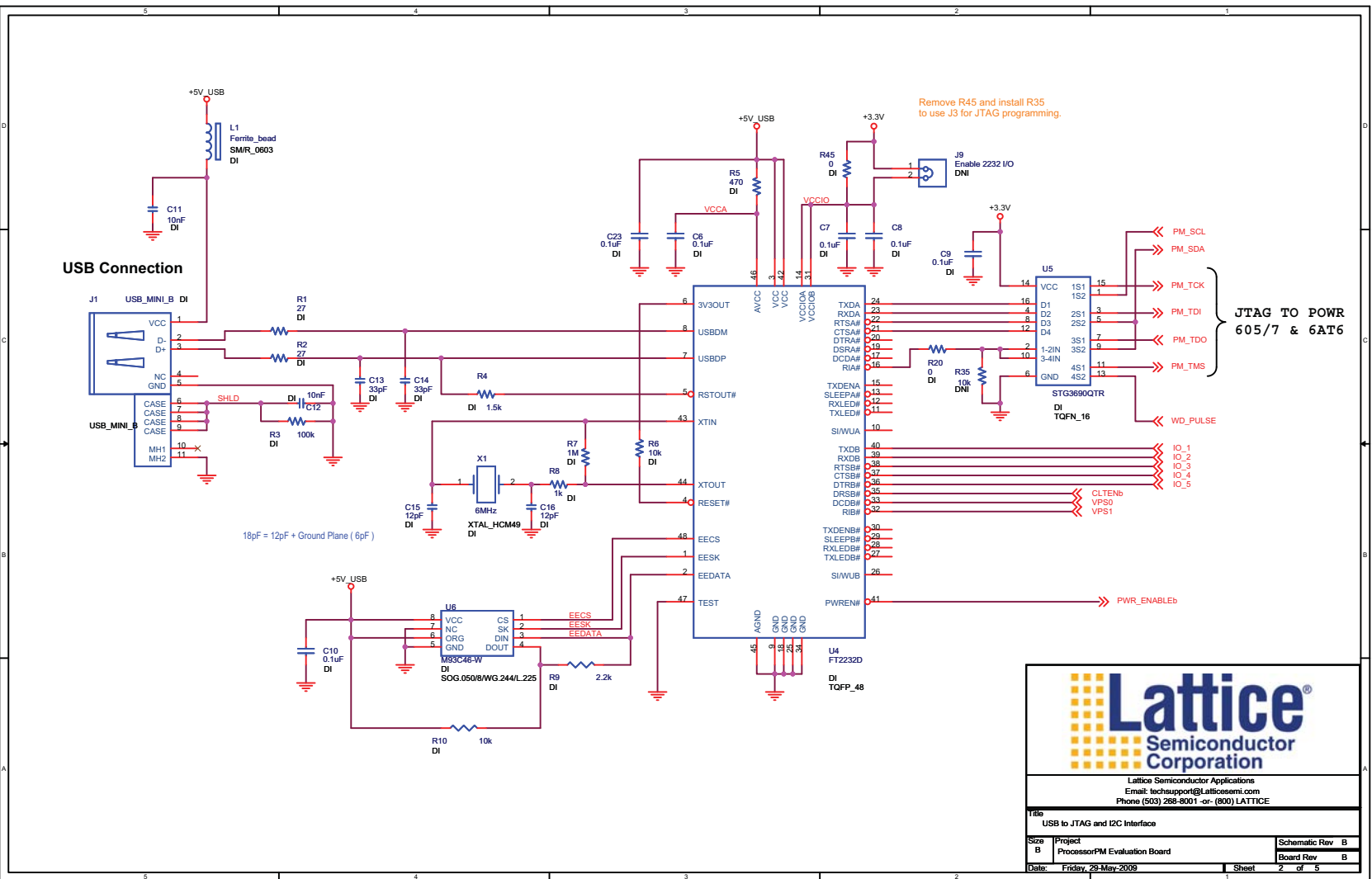
Figure 6. USB to JTAG and I 2 C Interface
