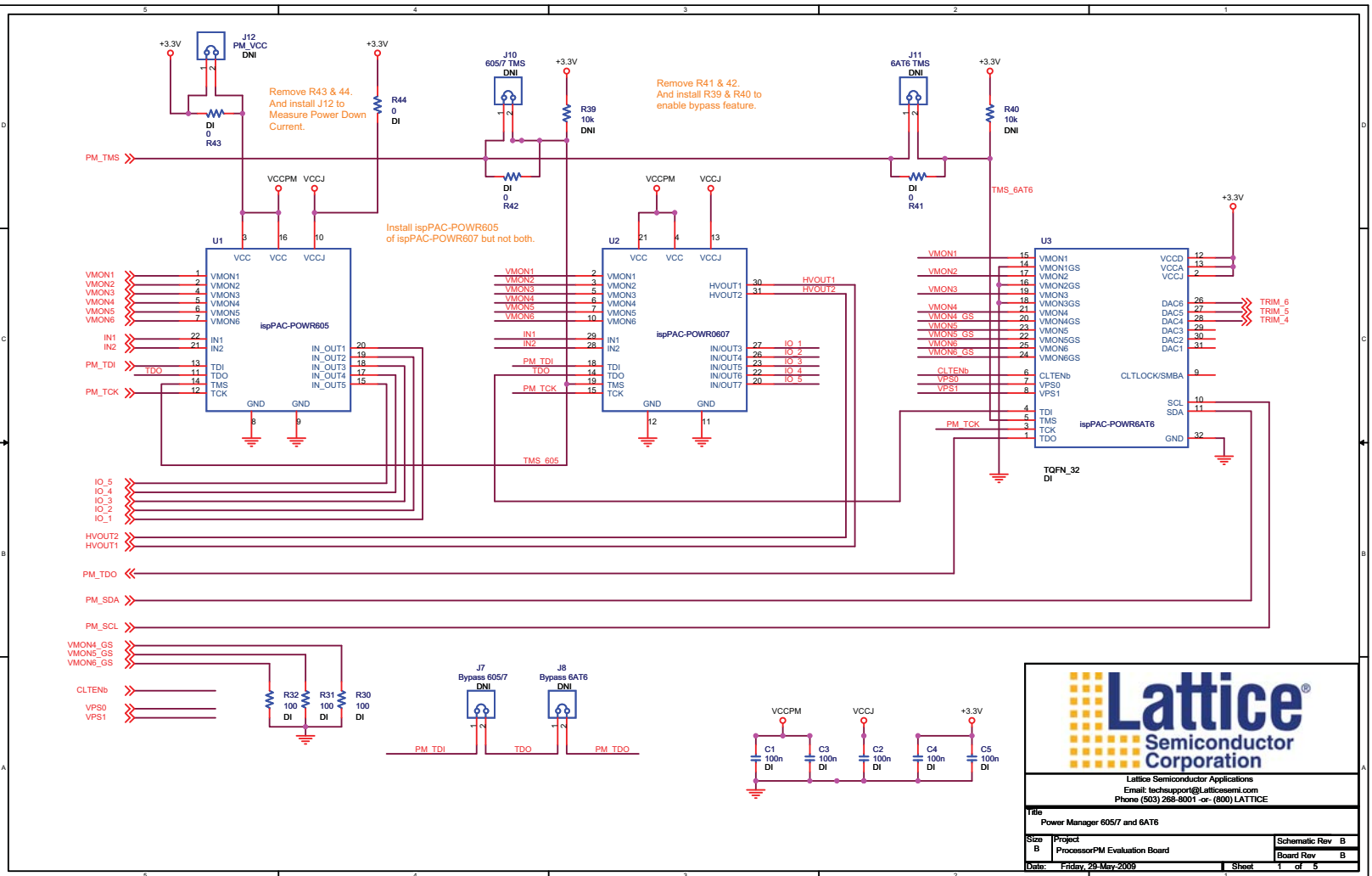
Figure 5. Power Manager 605/7 and 6AT6
