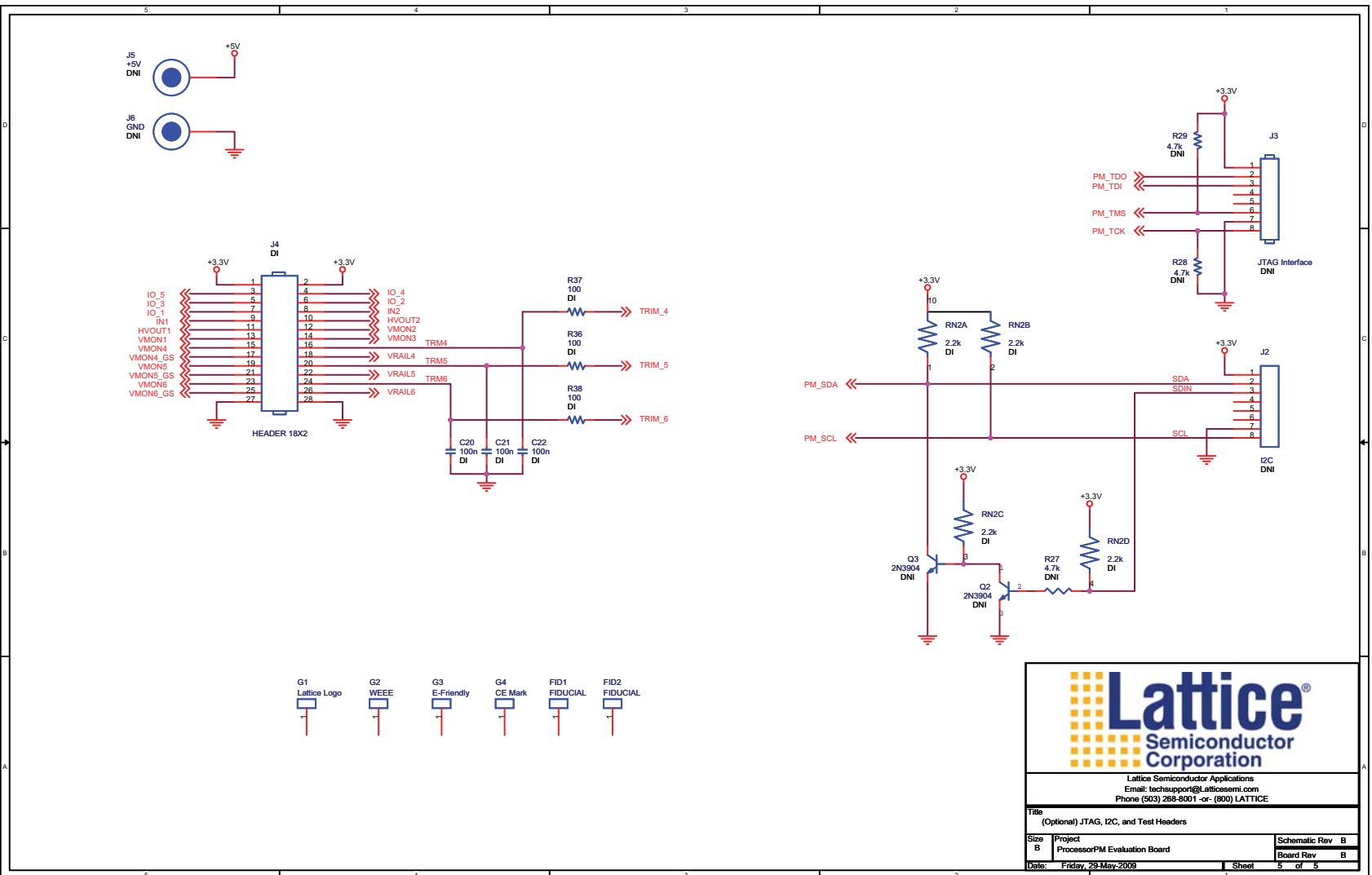
Figure 9. (Optional) JTAG, I 2 C and Test Headers
