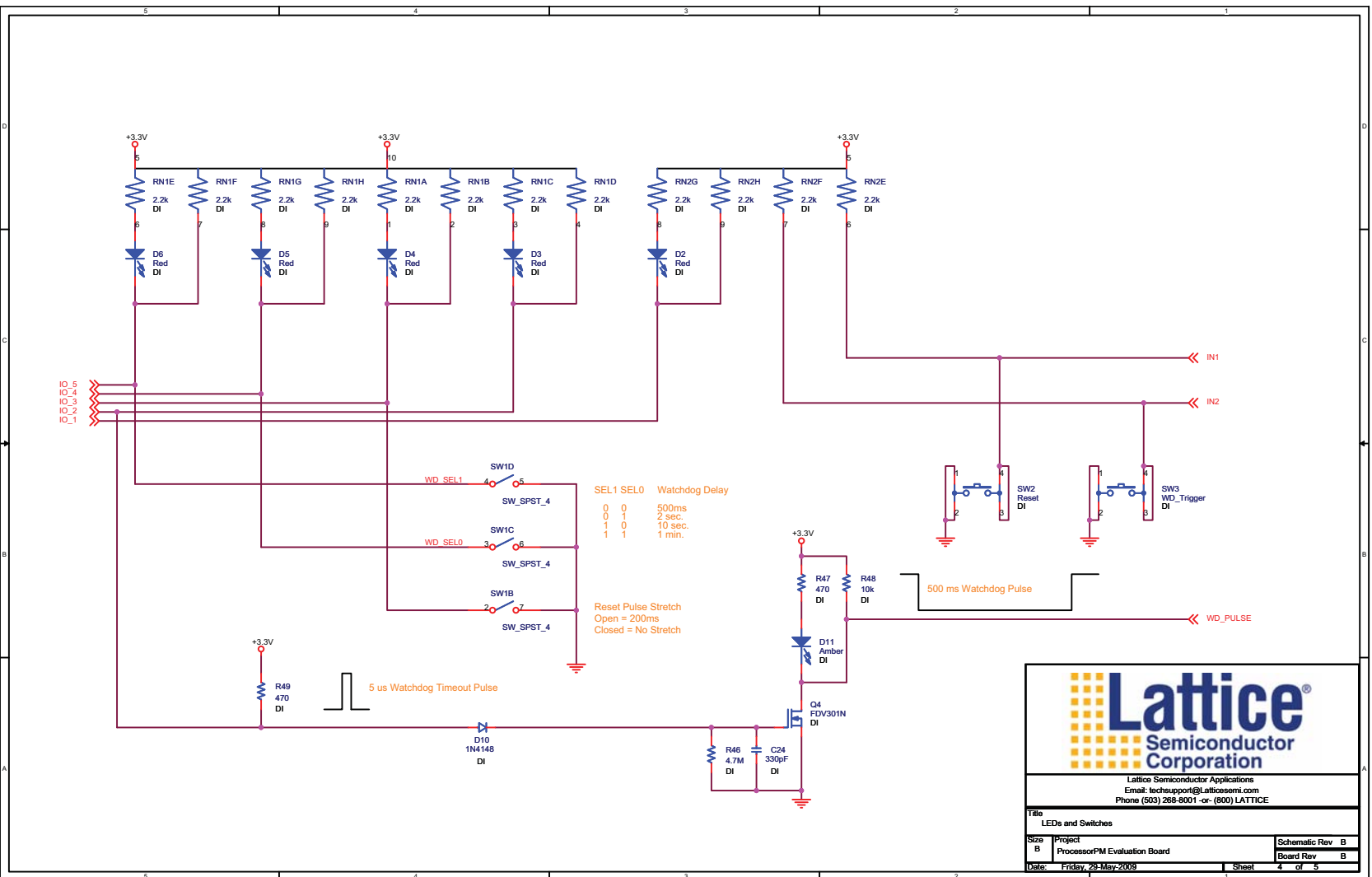
Figure 8. LEDs and Switches
