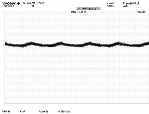
Figure 6: Output ripple & noise at 110/220Vac, 25A Iout VOUT: 100mV/div, 5mS/div
