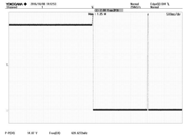
Figure 7: Output over voltage protection at 110/220Vac, 25A Iout VOUT: 2V/div, 500mS/div
