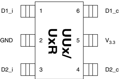
6-pin SC70
