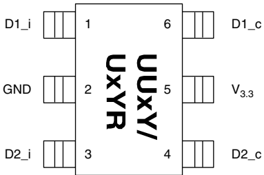
6-pin SOT23
