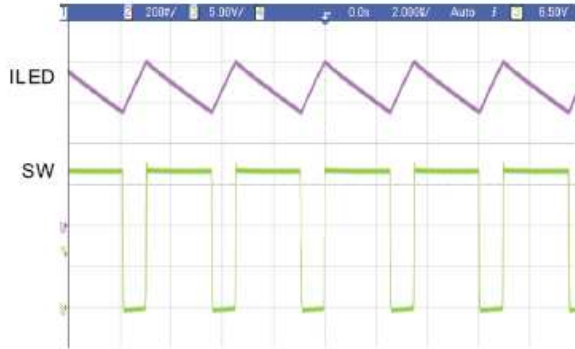
13. Steady State Waveforms
