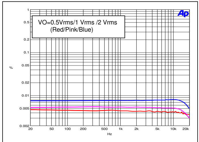
THD+N vs. Frequency (RL=600 \Omega )
