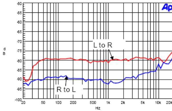
14. Crosstalk
