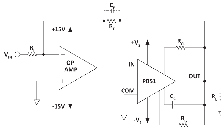
Figure 16: Typical Application
