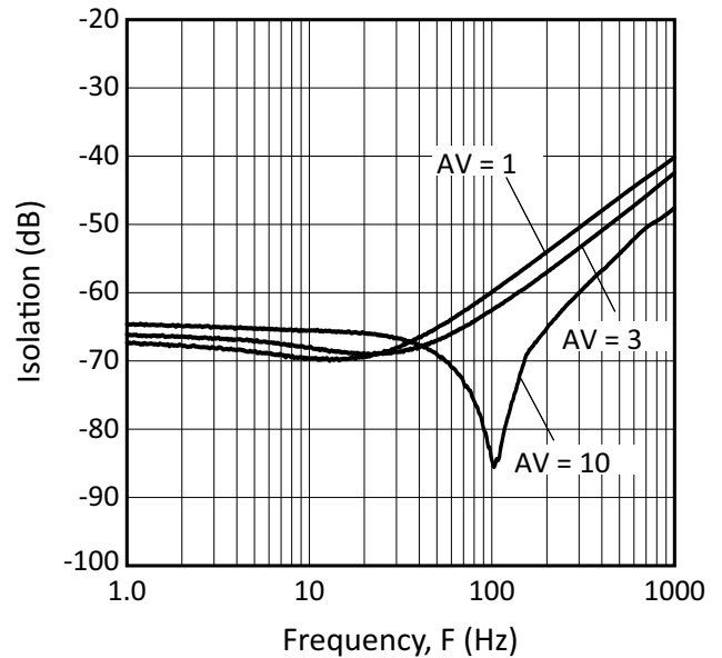
Figure 14: Channel Separation
