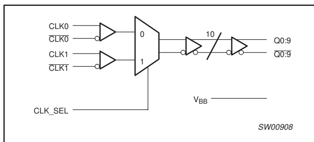
Figure 3. Logic symbol
