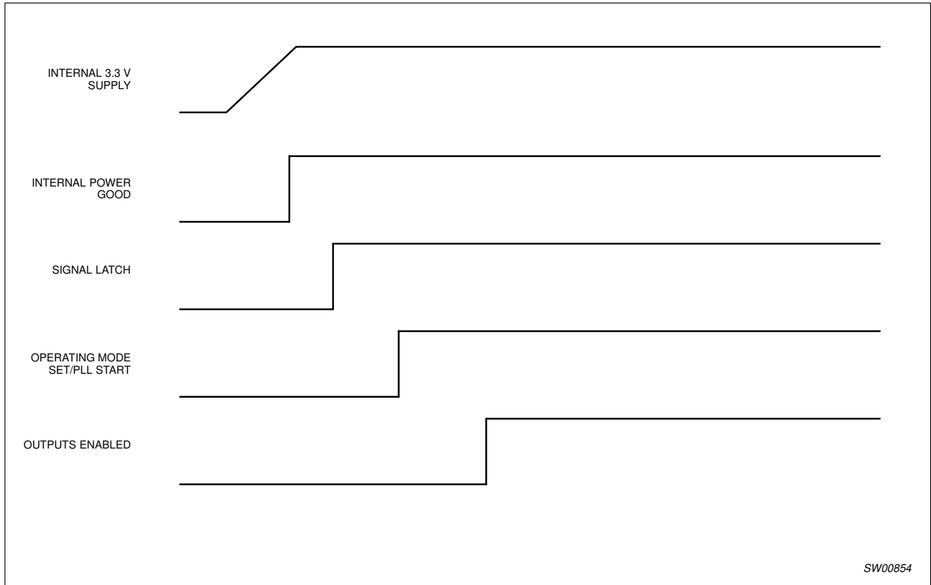
Figure 6. Power-up sequence
