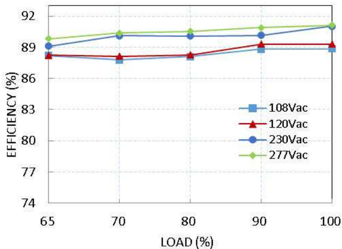
Efficiency vs. Load for PDA100B-700GB
