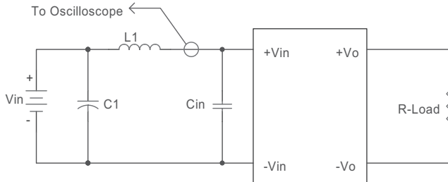
Figure 1 Measuring Input Ripple Current
