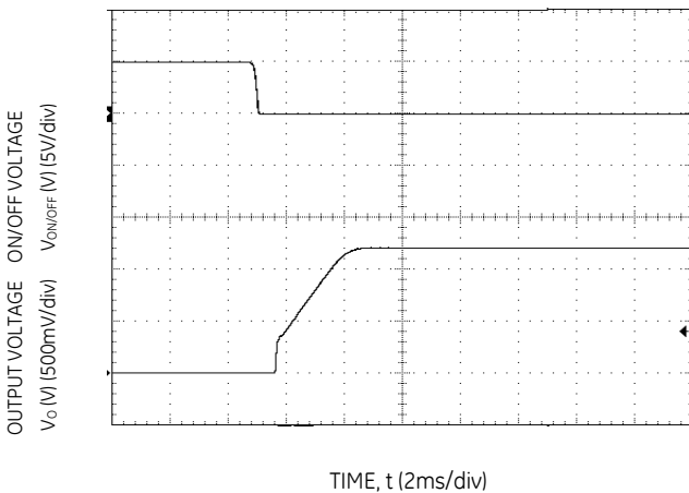
Figure 1. Typical Start-up Using On/Off Voltage (I o = I o,max ).
