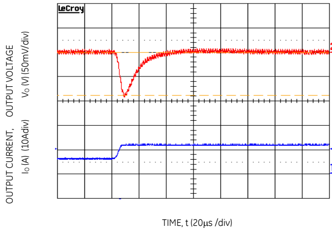
Figure 34. Transient Response to Dynamic Load Change from 50% to 100% at 12Vin, C_{out}= 5 \times 47\mu F , C_{Tune}=1500pF & R_{Tune}=330ohms
