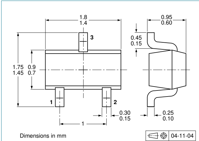
Fig 12. Package outline PDTA143EE (SOT416/SC-75)
