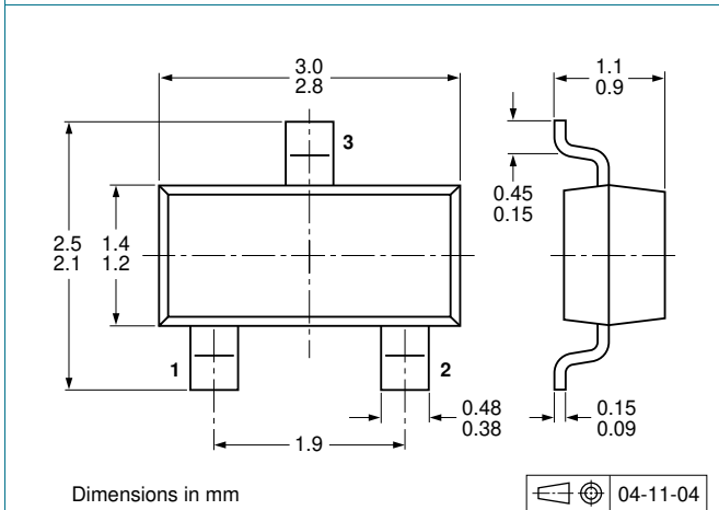
Fig 14. Package outline PDTA143ET (SOT23)
