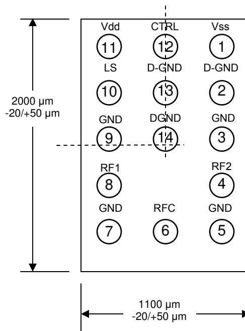
Figure 18. Pad Layout (Bumps Up)
