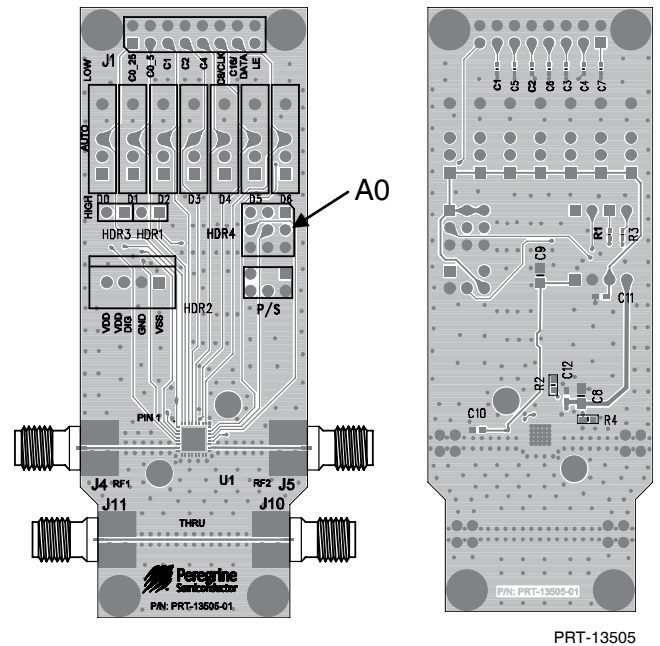
Figure 31. Evaluation Board Layout
