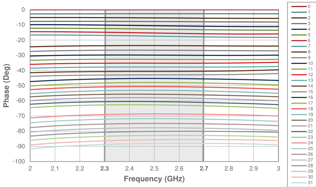
Figure 7 • Relative Phase RF_{IN}-RF_{OUT1} (All RF_{OUT1} Phase States)
