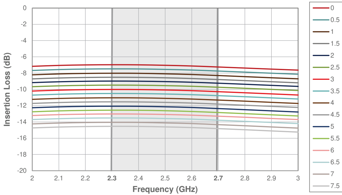
Figure 6 • Insertion Loss RF_{IN}-RF_{OUT2} (All RF_{OUT2} Attenuation States)
