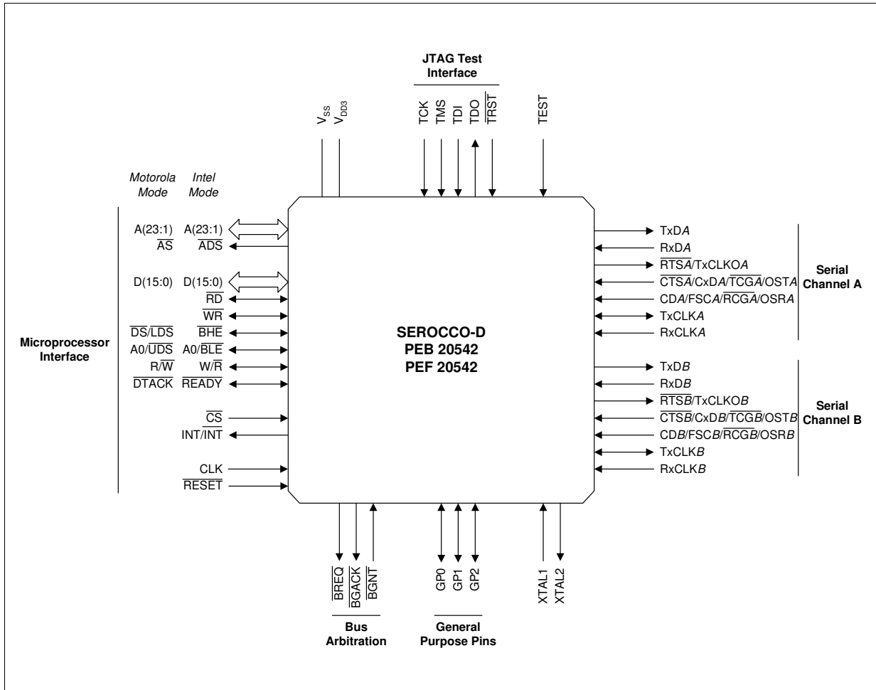
Figure 1 Logic Symbol
