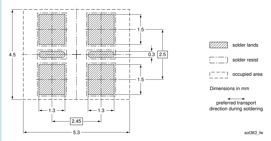
Fig 14. Wave soldering footprint PUMB15 (SOT363)
