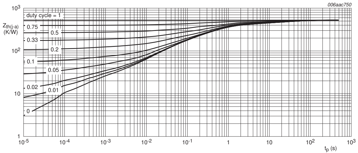
Fig 3. Per transistor: Transient thermal impedance from junction to ambient as a function of pulse duration for PUMD12 (SOT363); typical values
