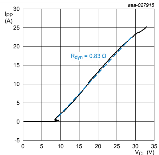
Fig. 4. Dynamic resistance with positive clamping; typical values; Input/output to ground
