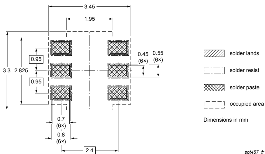
Fig. 11. Reflow soldering footprint for TSOP6 (SOT457)
