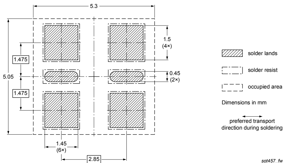
Fig. 12. Wave soldering footprint for TSOP6 (SOT457)
