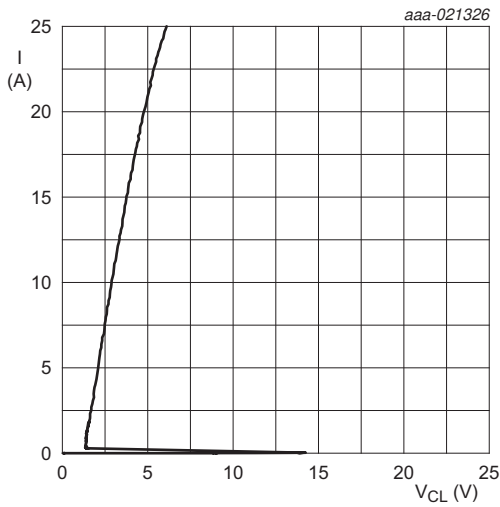
Transmission Line Pulse (TLP) = 100 ns
