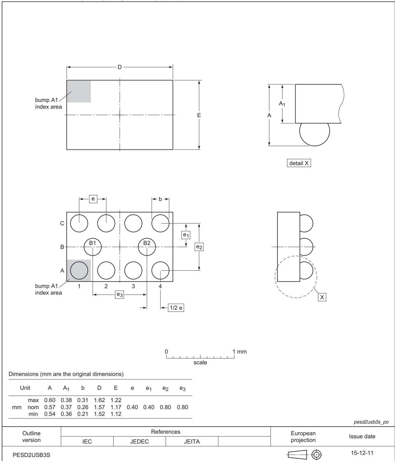
Fig 16. Package outline WLCSPP10
